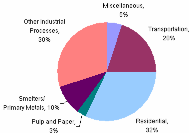
Figure 1: Ontario fine particulate matter (PM 2.5 ) emissions by sector, 2005
