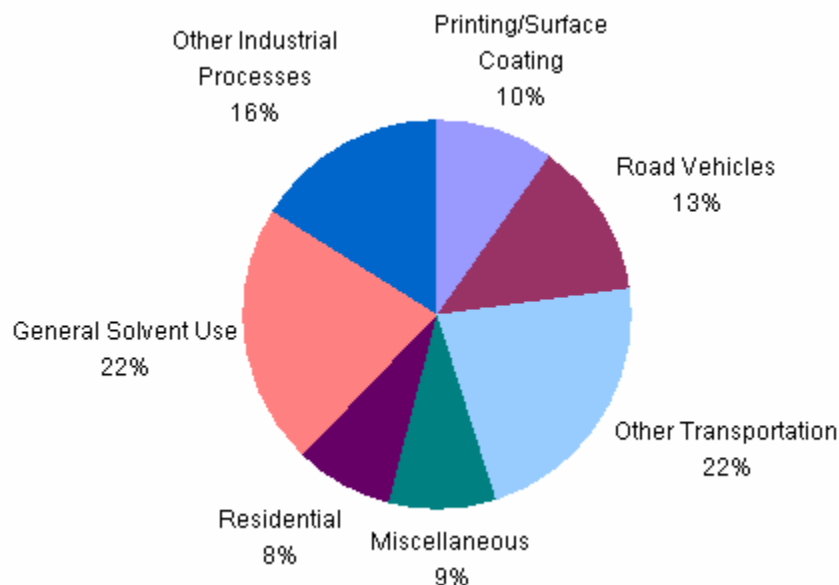
Figure 3: Ontario volatile organic compound (VOC) emissions by sector, 2005
