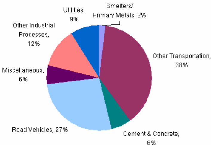
Figure 2: Ontario nitrogen oxide (NO x ) emissions by sector, 2005
