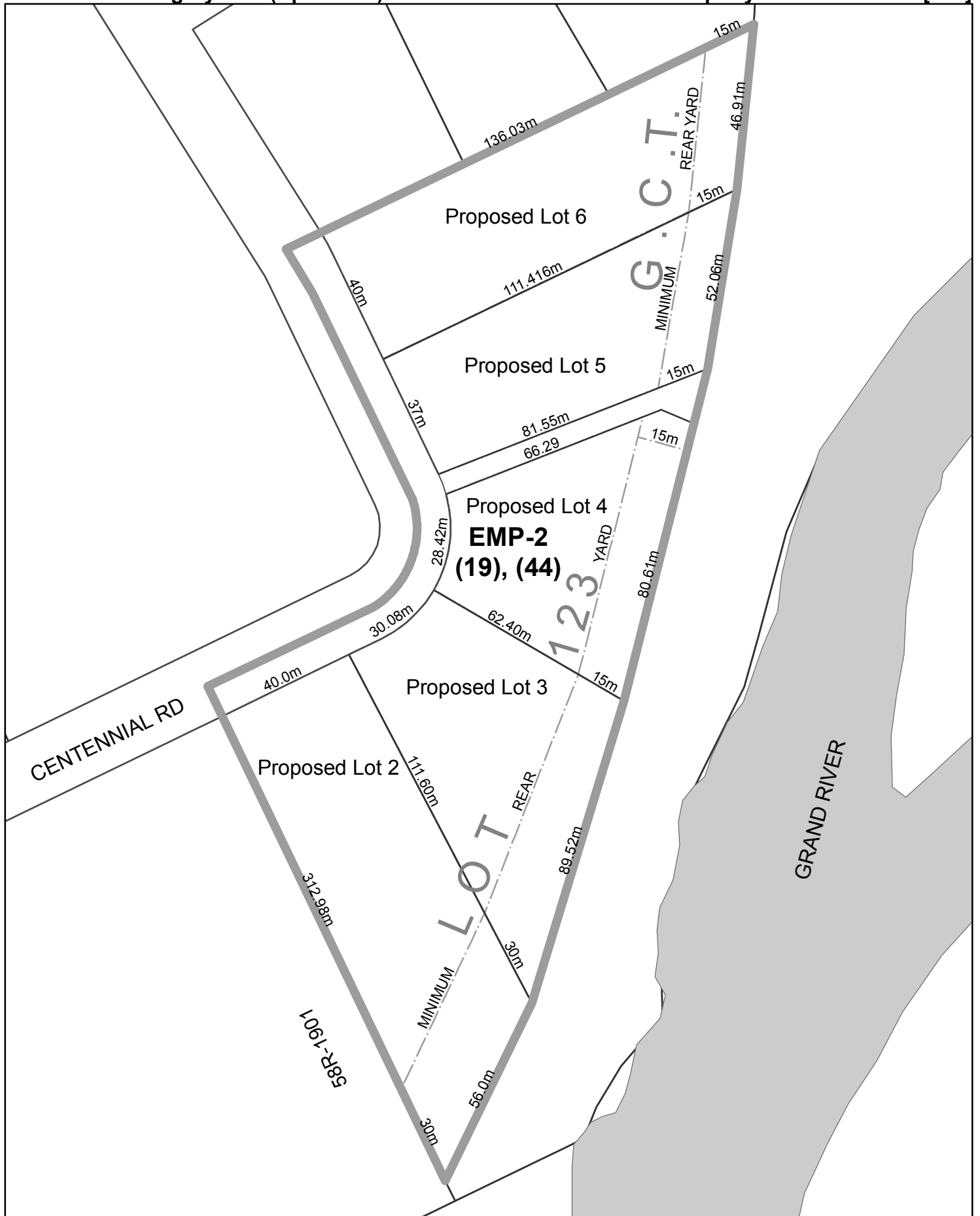
DETAIL from ZONING GRID SCHEDULE NO. 231 of APPENDIX 'A' SHOWING PART LOT 123 G.C.T.
