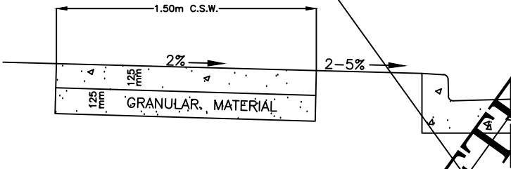
CROSS SECTION OF COMBINED WALK, BOULEVARD, CURB & GUTTER
